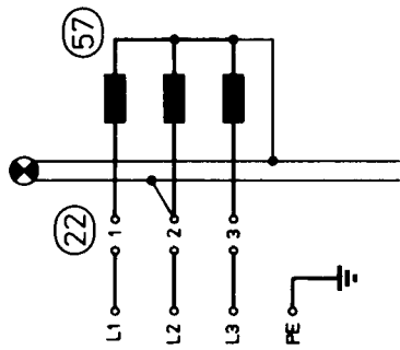
ART. 938 3x380V 50Hz
